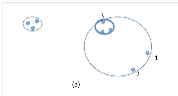
Figure 1: The k -means algorithm is extremely sensitive to outliers. By removing two points (1) and (2), we can obtain much tighter clusters (the bold circle near 3). The objective of this paper is to obtain a tight clustering and report the outliers in an automatic fashion.
