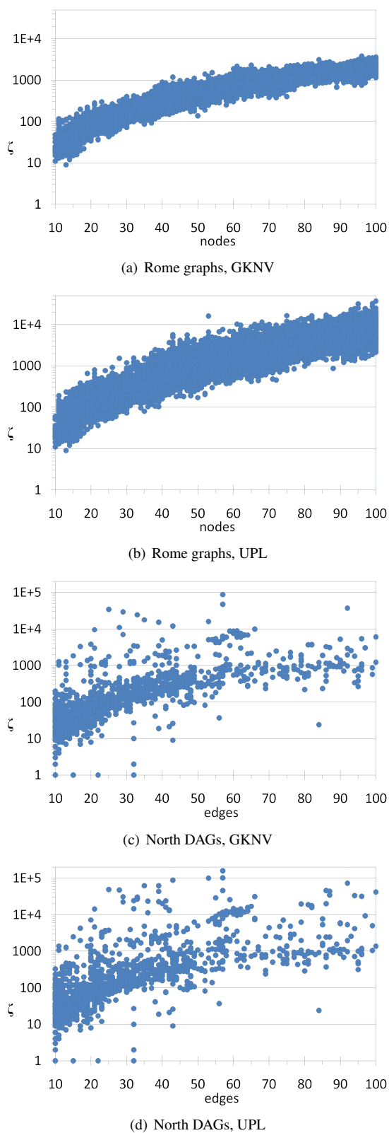
Figure 1: Correlation between original graph size and \zeta .
